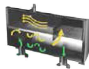
Condenser with integral economizer (patented) 250-550RT: built-in economizer; 600-1300RT: external economizer
